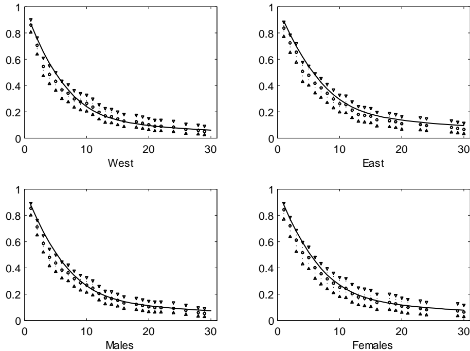
Figure 7 Kaplan-Meier and predicted survivor functions
