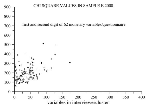
FIGURE 43: First two digit distribution: Chi-Square values for interviewer cluster in wave 3, sample E
