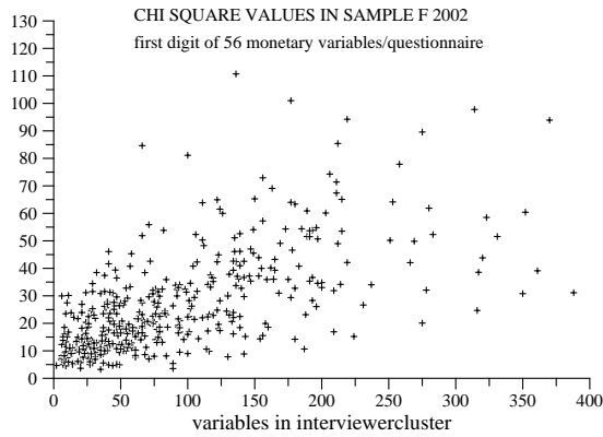
FIGURE 50: First digit distribution: Chi-Square values for interviewer cluster in wave 3, sample F
