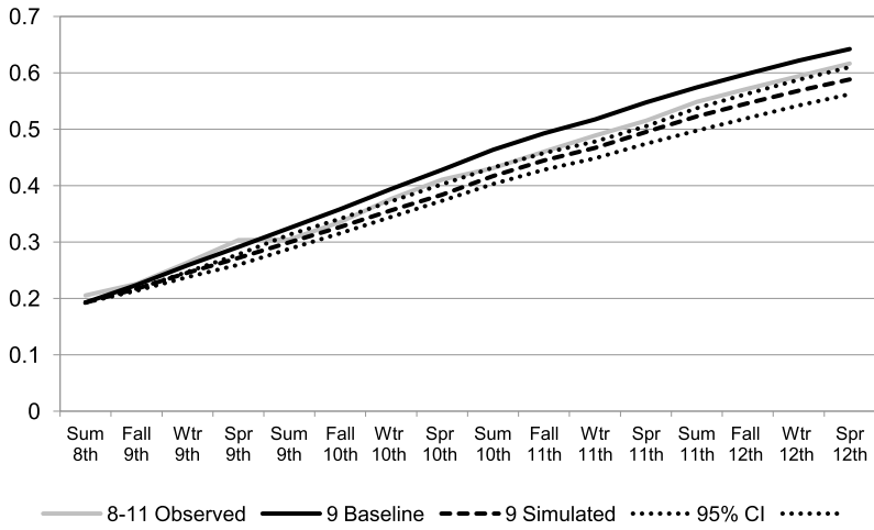
FIGURE 4. Eliminated effect of opposite-gender search behavior on arrival rates. “8–11 Observed” is 8th–11th grade cohorts, combined; “9 Baseline” is the prediction for the 9th grade cohort from estimated model; “9 Simulated” is the prediction from modified model.
