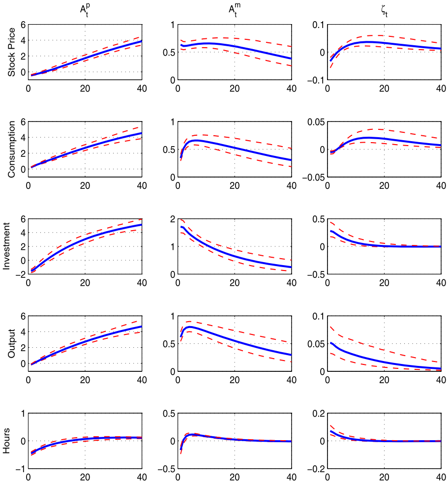
FIGURE 2. Impulse responses to a 1-standard-deviation permanent TFP shock ( A_t^p ), transitory TFP shock ( A_t^m ), and financial shock ( \zeta_t ) in the baseline model. All vertical axes are in percentage. We compute the responses for 20,000 draws from the posterior distributions. The solid line is the median value, the dashed lines indicate the 90 percent credible interval.
