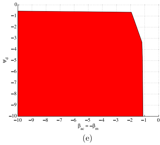
FIGURE 3. Two-dimensional representations of the confidence region at \beta_{00} = 1 , \mu = 0 , \sigma_\varepsilon = 1 , \sigma_u = 1 .
