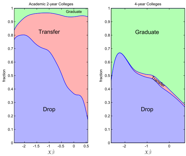
FIGURE 8. Empirical density of drop out, transfer, and graduate. NLS-72 cohort. As a function of ability measure X'\hat{\beta} and conditional on initial enrollment choice. First, a conditional (on the initial enrollment choice) nonparametric estimation of each event was performed. Next, each density was weighted by its share in initial enrollment. Finally, for every level of X'\hat{\beta} , the proportion of each event was constructed.
