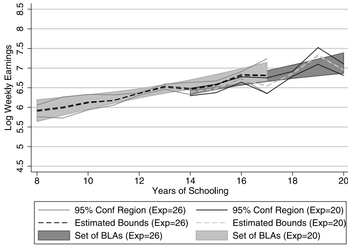
FIGURE 5. Nonparametric bounds on 1990 medians and best linear approximations for two experience groups of white men under S(F) \leq 0.05 .
