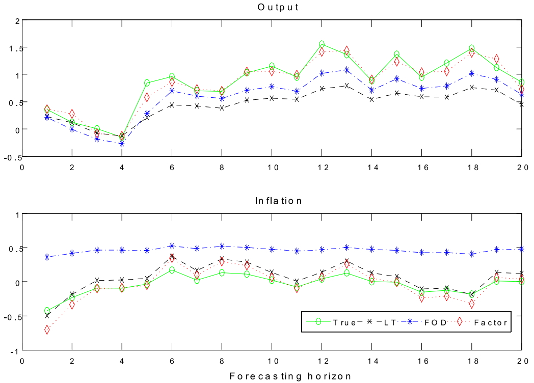
FIGURE 4. One-step-ahead forecasts, conditional on a constant interest rate path.
