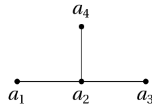
FIGURE 1. Tree G^T .
