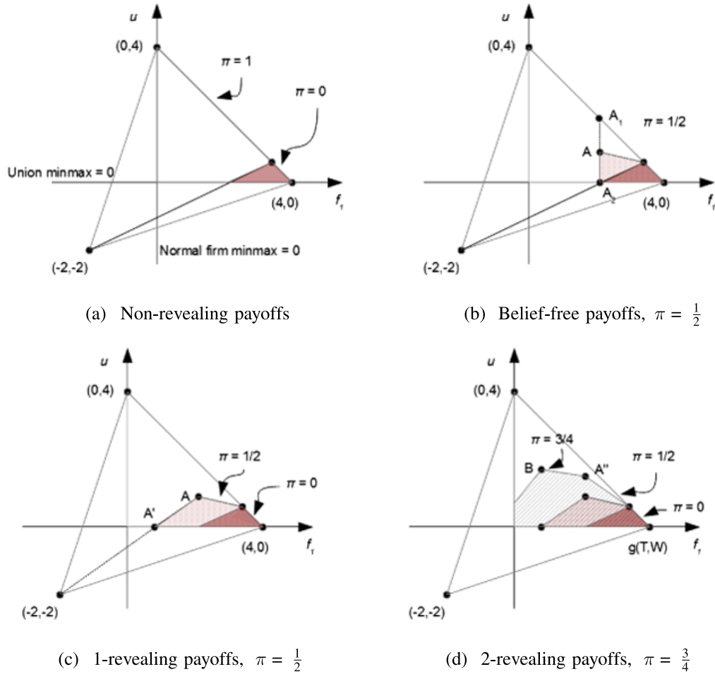
FIGURE 2. Finitely equilibrium payoffs in the union–firm bargaining.
