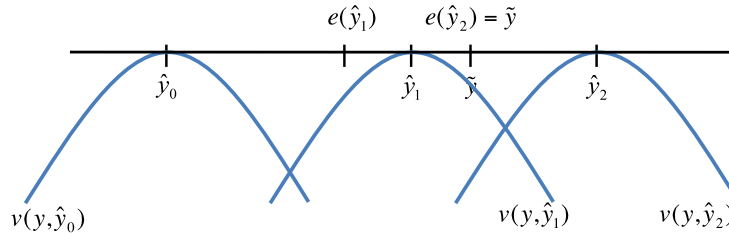
FIGURE 1. Illustration of e(\hat{y}_i) for i = 1, 2 when \hat{y}_1 < \tilde{y} < \hat{y}_2 .
