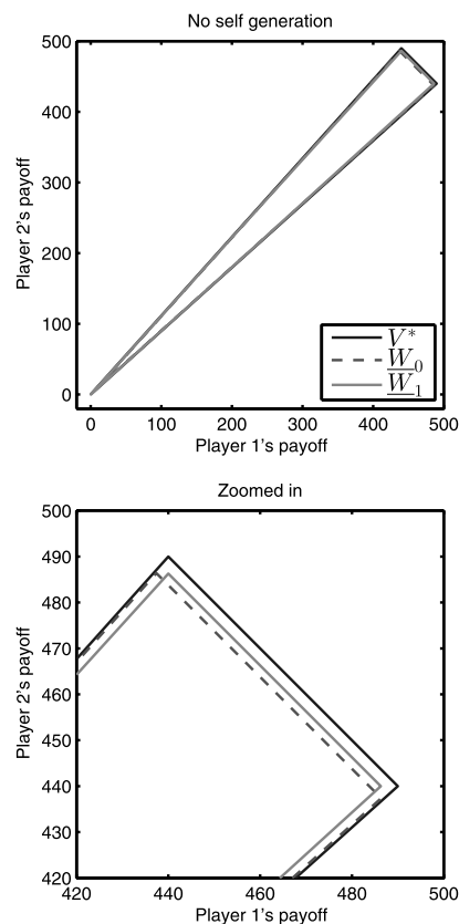
FIGURE 10. An example in which the set W_0 does not supergenerate.
