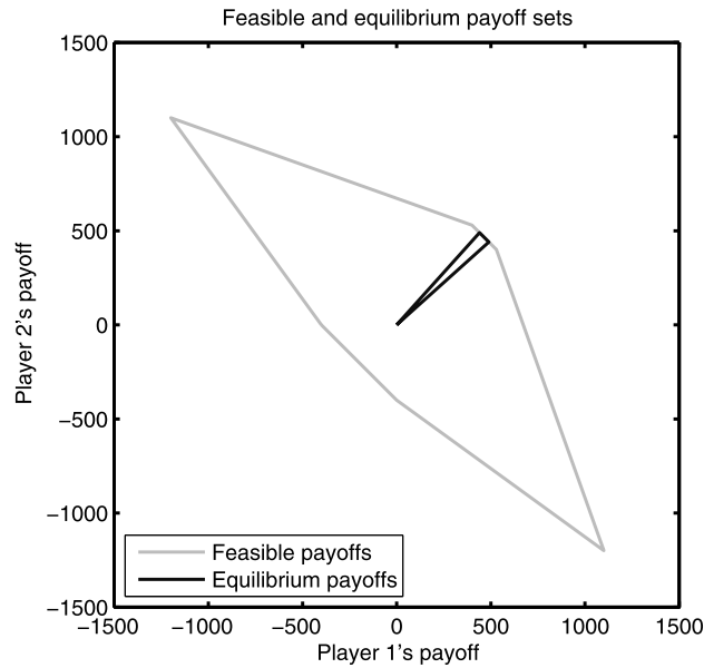
FIGURE 8. A narrow set V^* for \delta = 0.6 .
