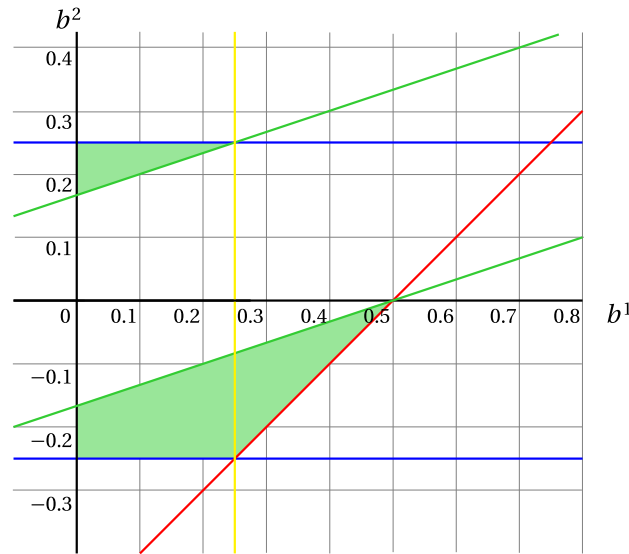
FIGURE 2. The parameter region for which 2-action mixed equilibria exist.
