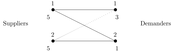
FIGURE 5. A new link may hurt noninvolved agents.
