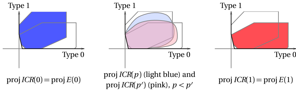
FIGURE 3. The sets \text{proj } ICR^*(p) for p \in [0, 1] .
