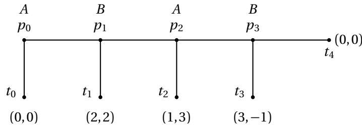
FIGURE 5. A finite horizon stopping game
