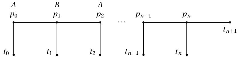
FIGURE 5. A finite horizon stopping game
