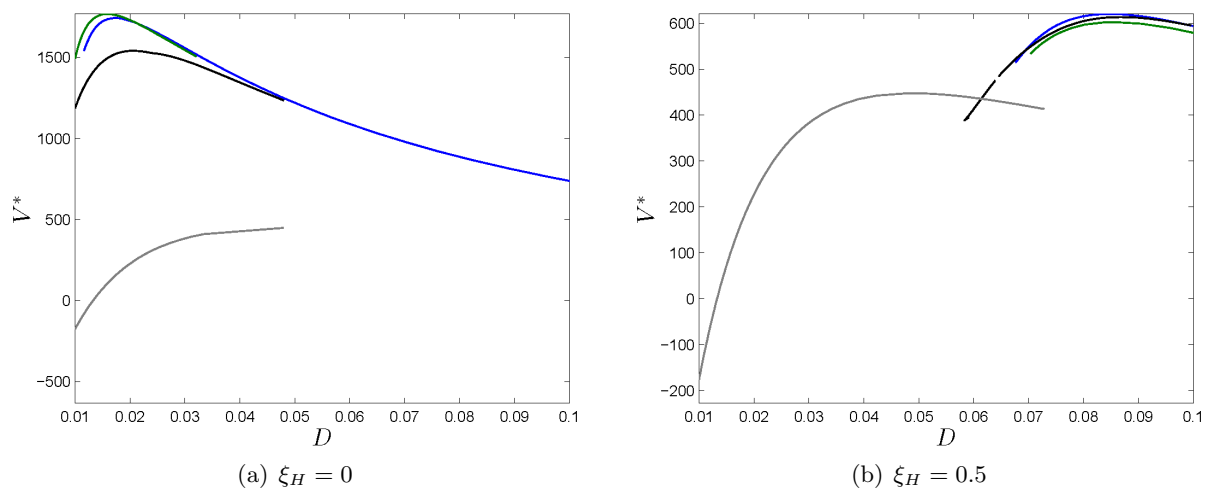
Figure 10: The net present value V^* depending on D for no impulse investments (grey), one impulse investment (black), two impulse investments (blue) and three impulse investments (green).
