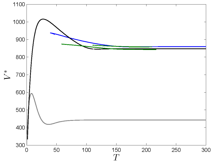
Figure 6: Solution structure given by the objective value V^* depending on the planning horizon T for no impulse investments (grey), one impulse investment (black), two impulse investments (blue) and three impulse investments (green)
