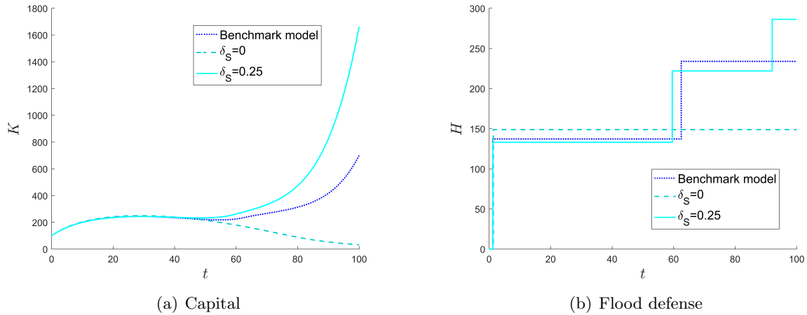
Figure 5: State dynamics for \delta_S = 0 (dashed blue line), \delta_S = 0.1 (dotted dark blue line) and \delta_S = 0.25 (solid light blue line) in the planning period [0, T] . If the salvage value of the firm is important (a) firm's capital K increases towards the end of the planning horizon and (b) firms invest more and more often in flood risk protection measures.
