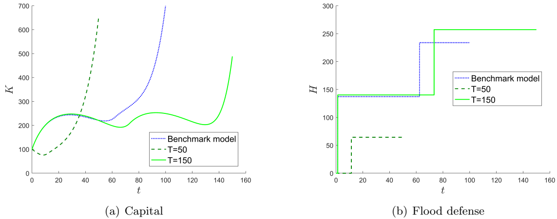
Figure 7: State dynamics for planning horizon T = 50 (dashed dark green line), T = 100 (dotted blue line) and T = 150 (solid light green line). If the planning horizon T is longer (a) firms invest more in capital K even in the beginning and (b) firms invest more and more often in flood risk protection measures.
