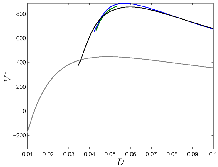
Figure 4: Solution structure given by the objective value V^* depending on D for no impulse investments (grey), one impulse investment (black), two impulse investments (blue) and three impulse investments (green).
