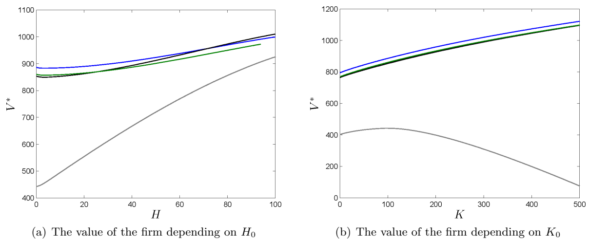
Figure 9: The net present value V^* of the firm increases for higher initial capital stocks. The colors indicate no impulse investments (grey), one impulse investment (black), two impulse investments (blue) and three impulse investments (green).
