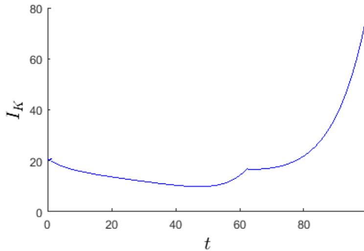
Figure 3: Capital investment I_K
