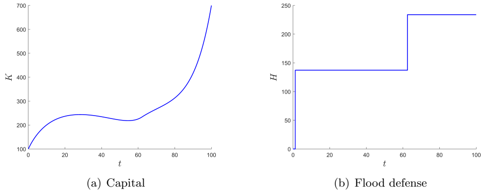
Figure 2: State dynamics in the planning period [0, T] . Firm's capital K (a) increases only when the flood risk is low in consequence of a high flood risk protection standard (b).
