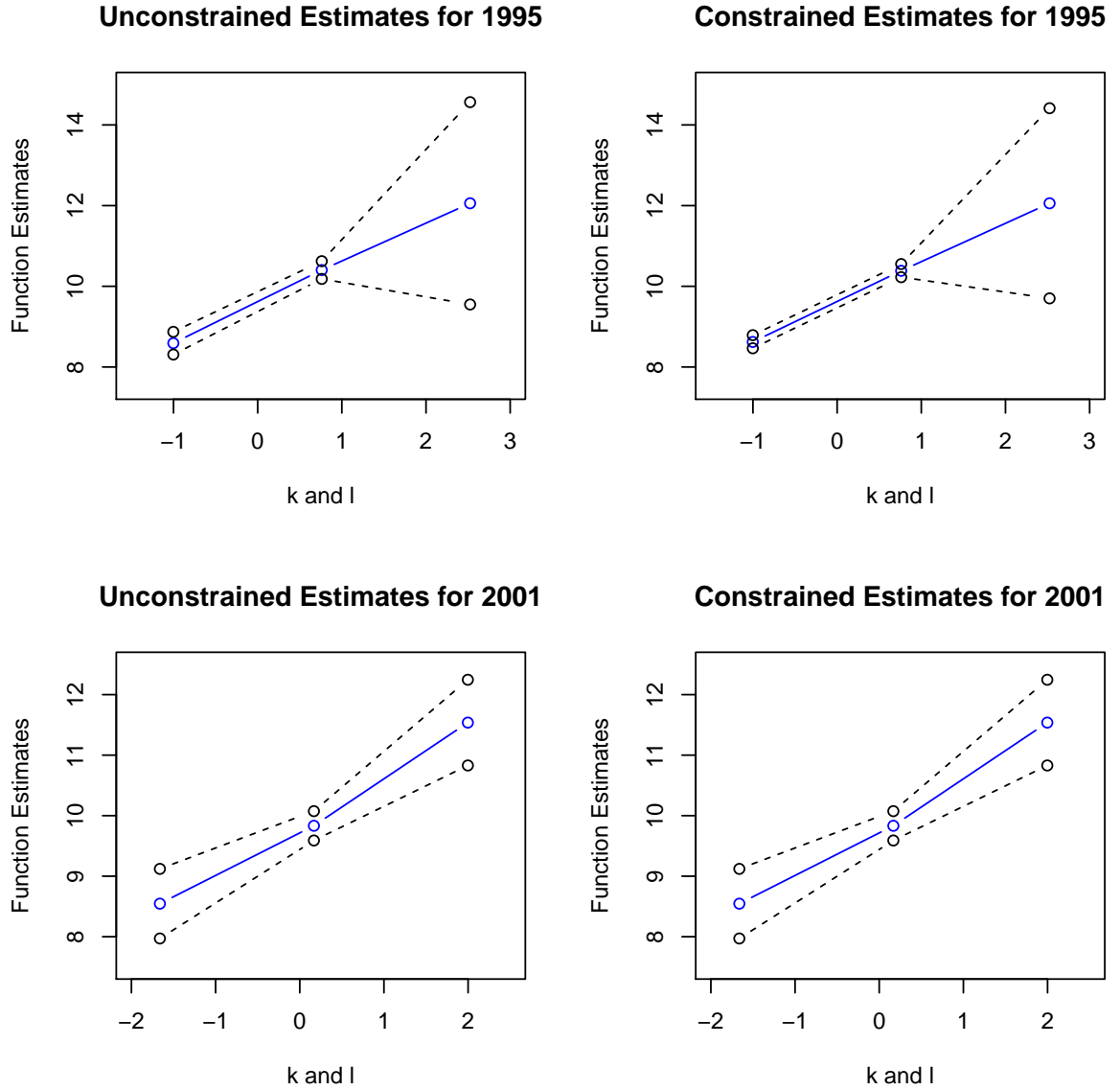
FIGURE 2. Nonparametric Estimates and their Uniform Confidence Bands (Bias Correction Implemented)
