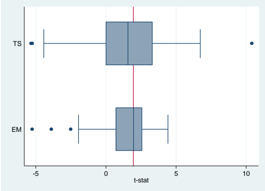
Figure 1: Boxplot for the classification of the dependent and independent variable
