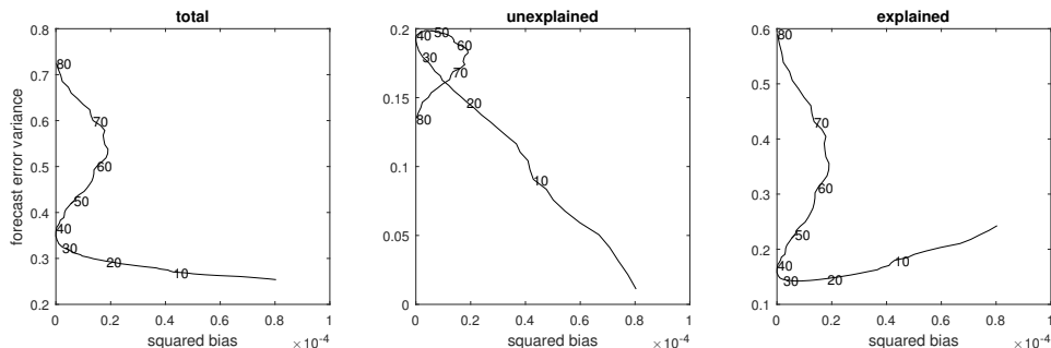
Figure 7: Bias-variance Trade-off
