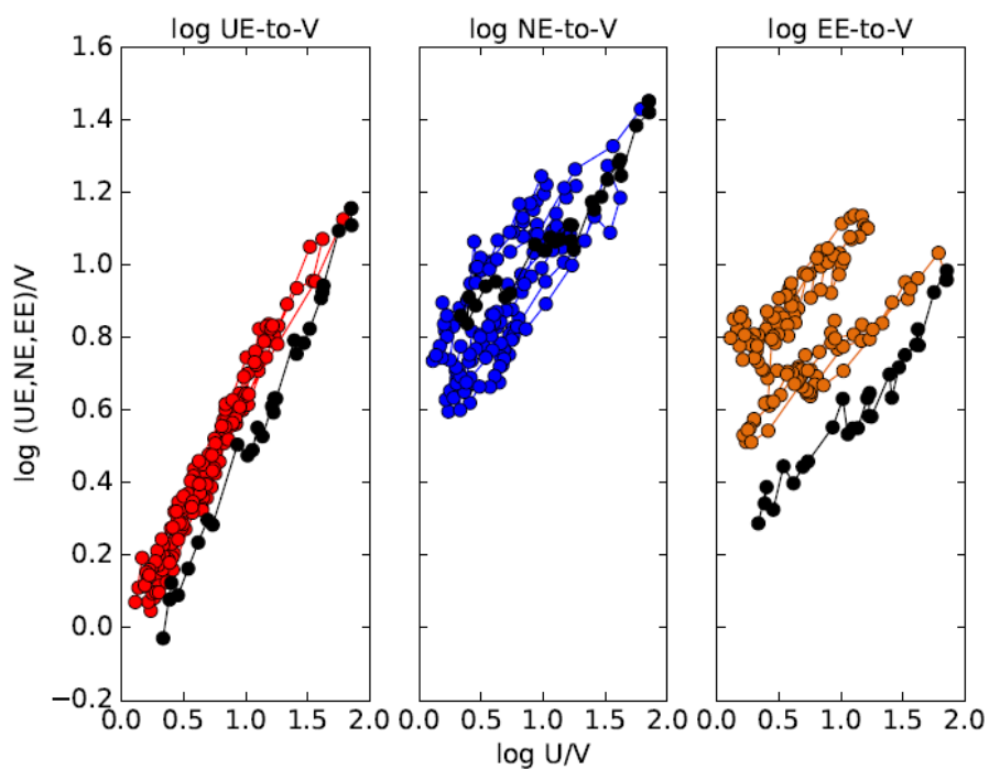
Figure 9. Matching Function Regression Residuals
