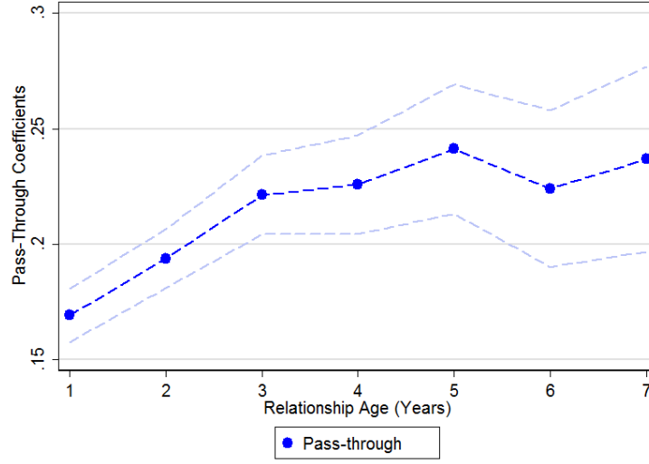
Figure 2: Cross-sectional pass-through regressions
