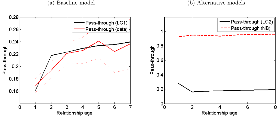
Figure 7: Pass-through by relationship age
