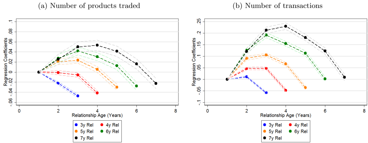
Figure F.12: Relationship life cycle
