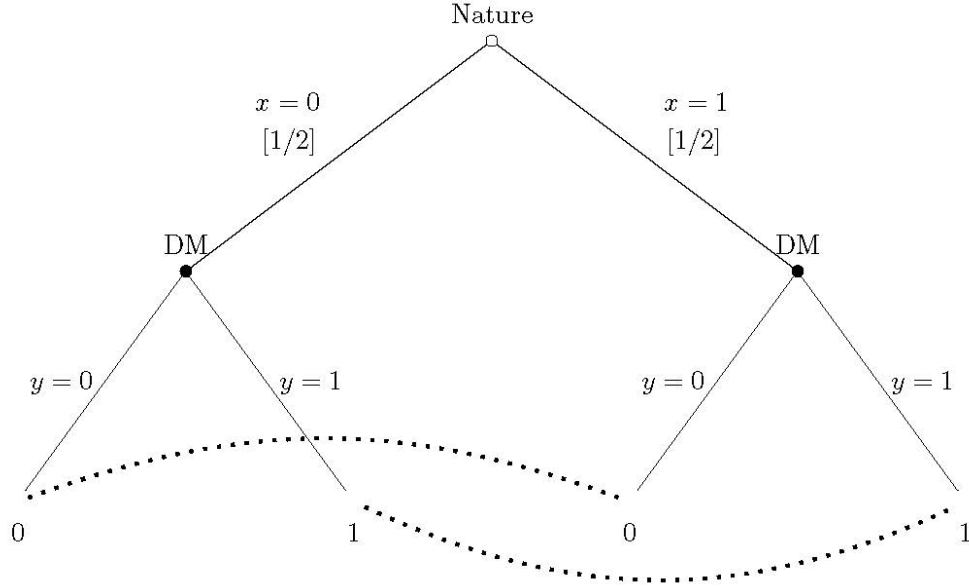
Figure 1, n=1 (coin-flip)
