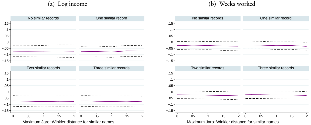
Figure A6: Measurement Error Due to Matching – Similarity of Names
