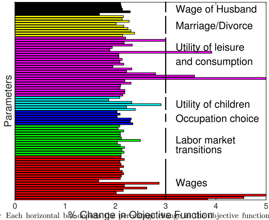
Figure A1: Sensitivity of the objective function with respect to model parameters
