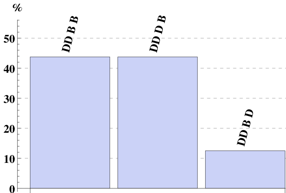
Figure 11: Robustness check
