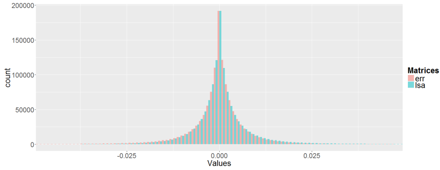
Fig. 33 Histograms of D_k and D_{err}
