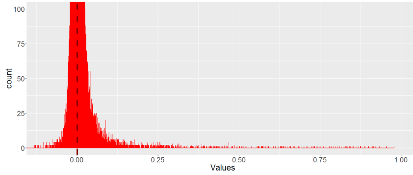
Fig. 38 Histogram of the full semantic kernel U_k U_k^T
