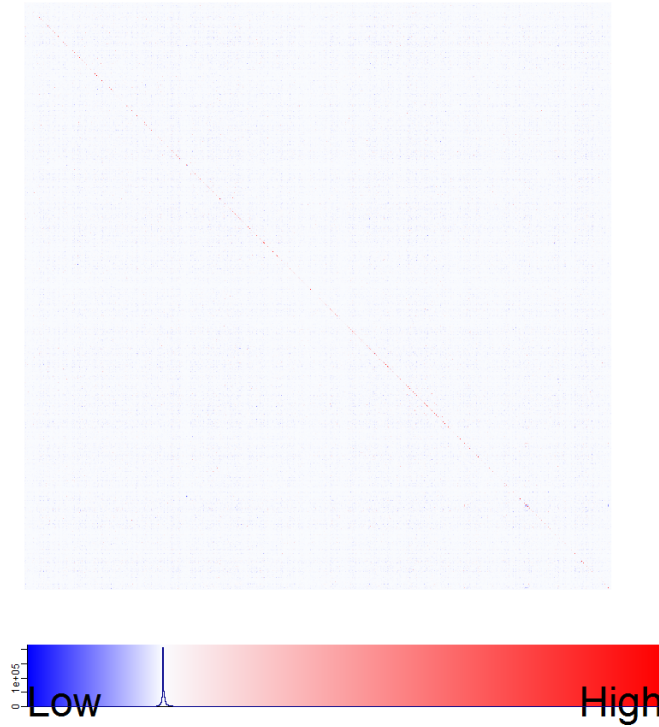
Fig. 39 Heat map of the full semantic kernel U_k U_k^T
