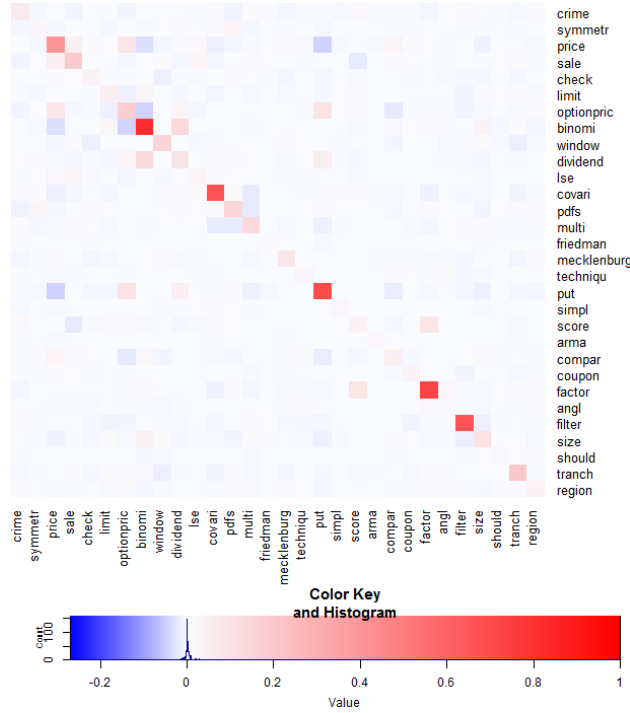
Fig. 37 Heat map of semantic kernel U_k U_k^\top , random subset 30 \times 30
