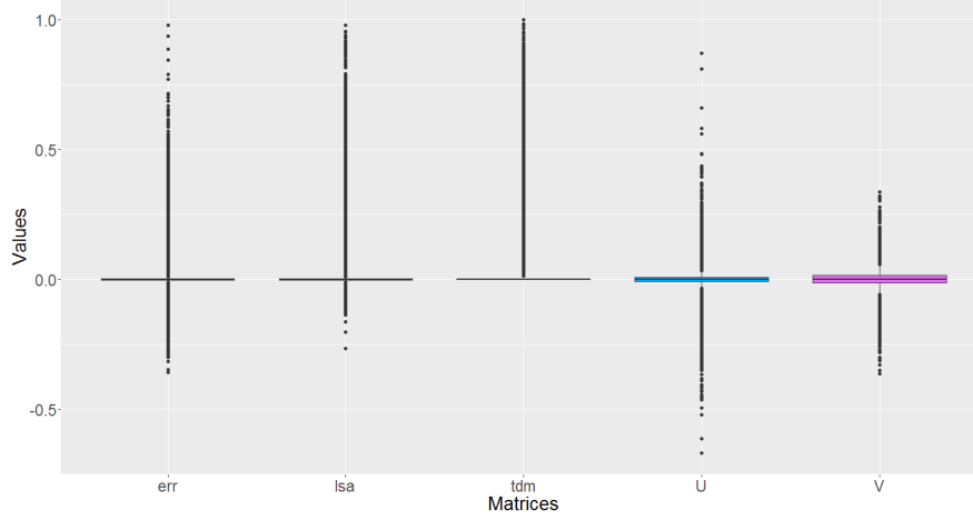
Fig. 36 Boxplots of D_{err} , D_k , D , U_k^\top , V_k^\top
