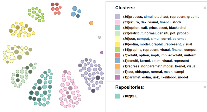
Fig. 23 SFE Quantlets clustered by k -means into 12 clusters, the tooltip on the right shows their topics
