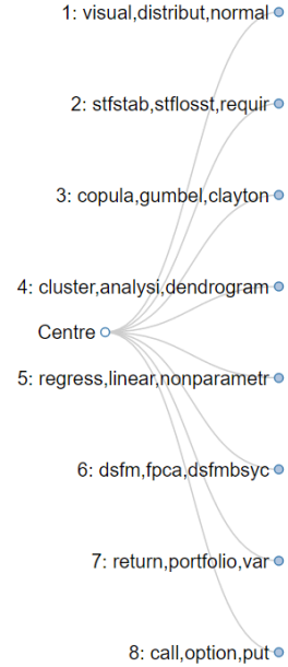
Fig. 40 Topics of the first 8 “semantic components” (LSA on the left) versus cluster labels of the dendrogram (HC on the right)
