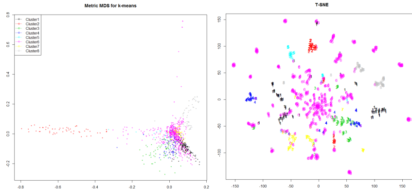
Fig. 19 LSA:50 geometry of Quantlets via MDS (left) and t-SNE (right), clustered by k -means with generated topics
