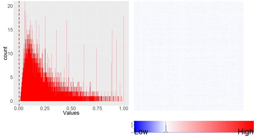
Fig. 32 Histogram of the matrix values in D (to the left); heat map with color key of the error matrix D_{err} (to the right)
