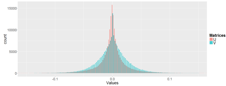
Fig. 35 Histograms of U_k^\top , V_k^\top
