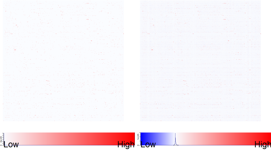
Fig. 31 Heat maps with color key of D and D_k (from left to right)
