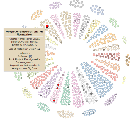
Fig. 13 Orbit clustering of QuantNet, LSA model, k -means, 40 clusters. Quantlets containing the search query “big data” highlighted in red
