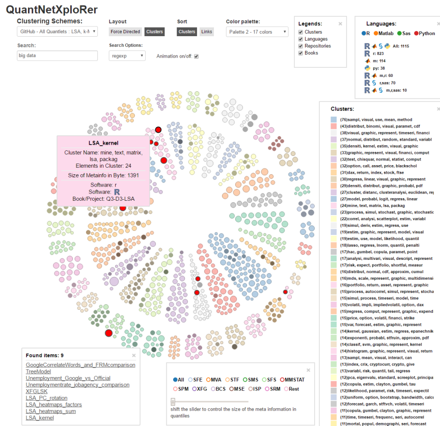
Fig. 41 Front end view: all Quantlets in QuantNetXploRer, search term “big data”
