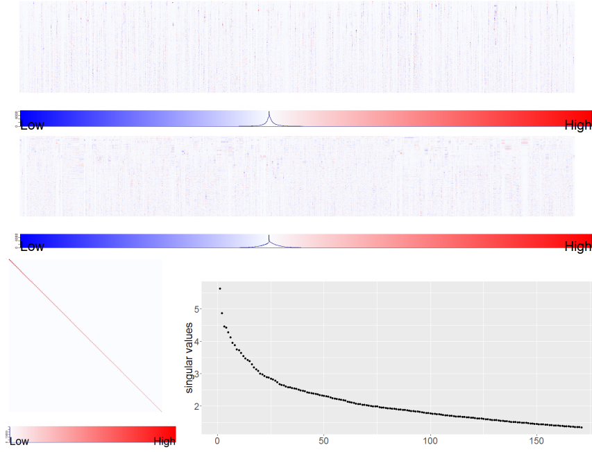
Fig. 34 Heat maps of U_k^\top , V_k^\top , \Sigma_k (from top to bottom); plot showing the highest singular values having a total sum of 50%
