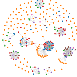
Fig. 4 Galaxy MVA with clusters
