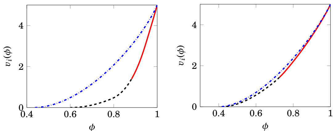
(a) Bolton and Harris (1999); \phi^* = 0.43 \bar{\phi} = 0.60 . (b) \lambda = 0.1 , \gamma = 1 ; \phi^* = 0.40 \bar{\phi} = 0.73 , \bar{\bar{\phi}} = 0.41 .
