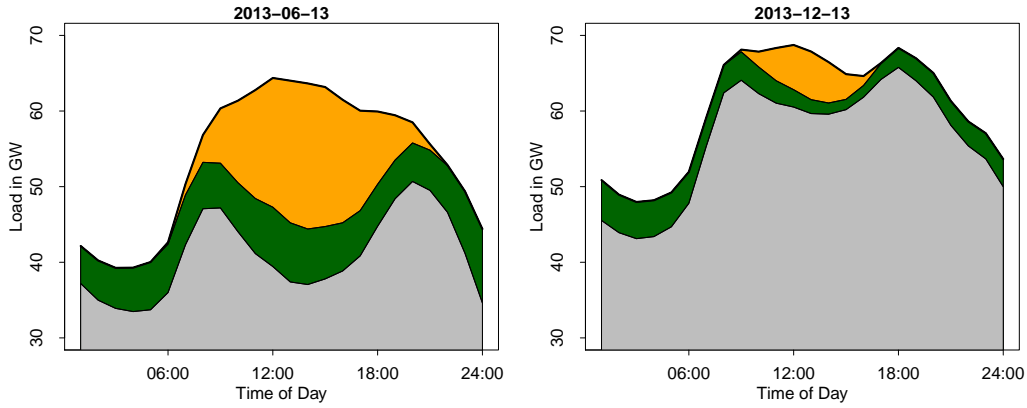
Figure 3: Total consumption (thick black line), solar infeed (orange), wind infeed (green) and residual load (gray) on a day with high renewable infeed (left) and low renewable infeed (right).
