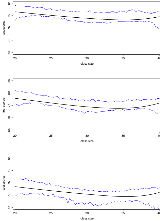
Figure 2: Estimated structural effects (thick line) for q \in \{0.25, 0.5, 0.75\} and 90% confidence intervals (blue lines)
