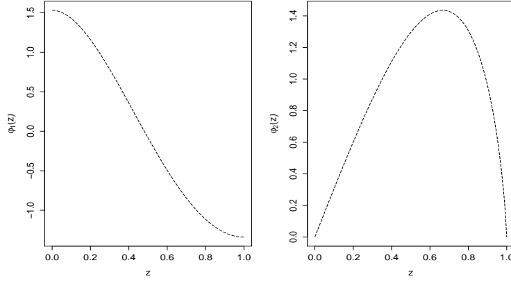
Figure 1: Graphs of \varphi_1 and \varphi_2
