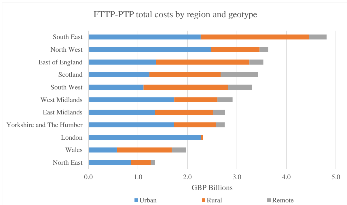
Figure 7 FTTP-PTP total costs per region and geotype
