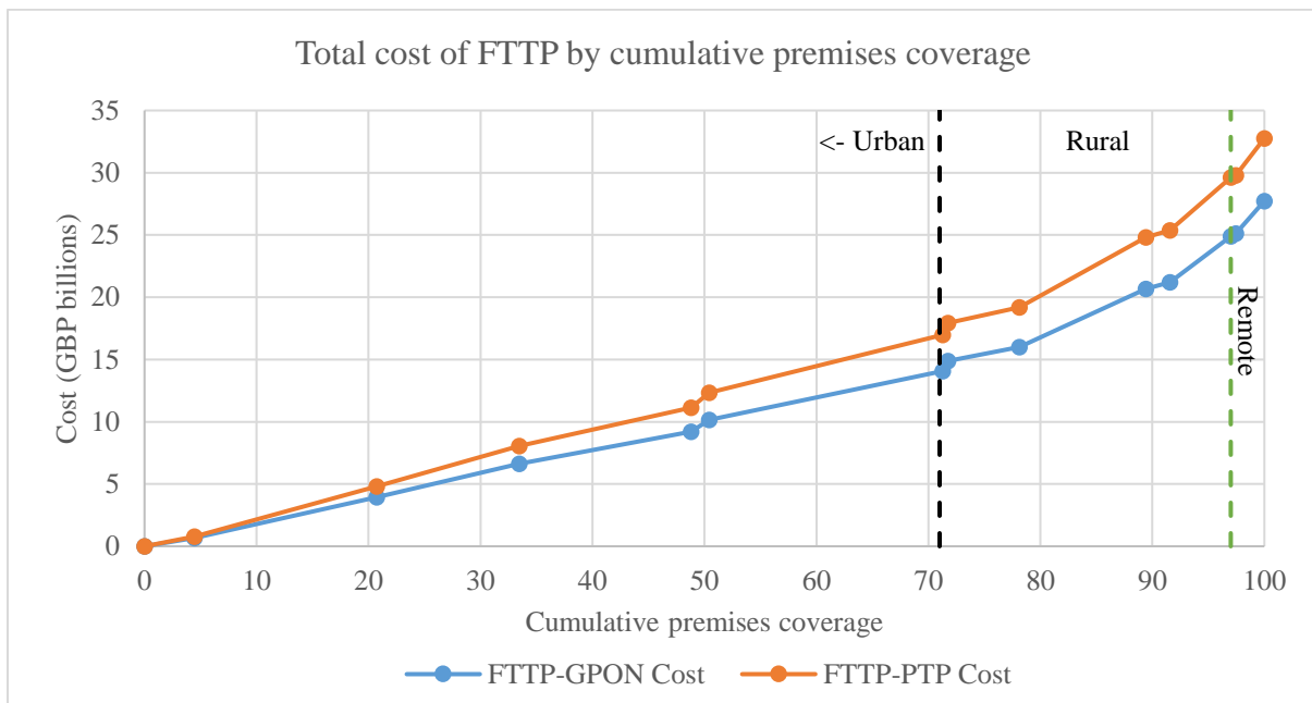
Figure 5 Total cost of FTTP technologies vs. premises coverage
