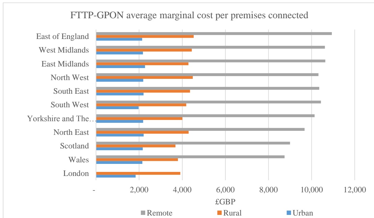
Figure 3 FTTP-GPON average marginal cost per premises connected by region and geotype
