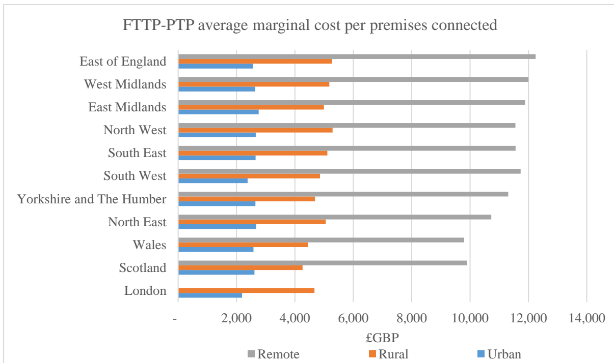
Figure 4 FTTP-PTP average marginal cost per premises connected by region and geotype
