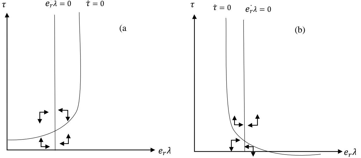
Figure 2: Phase diagrams for e_r\lambda^* and \tau^* , stable and unstable case
