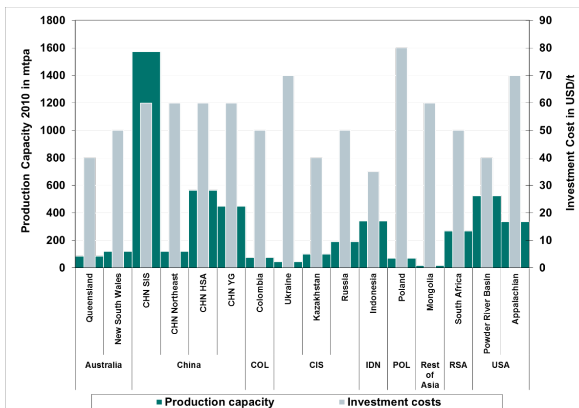
Figure 9: Capacity and investment costs for all production nodes in the base year.
