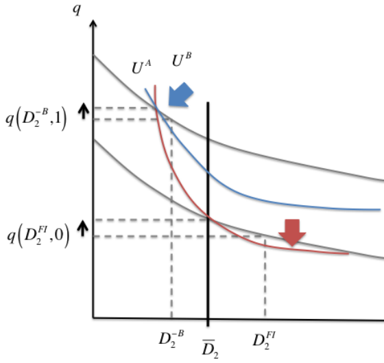
Figure 8: Separating equilibrium with a common debt ceiling.
