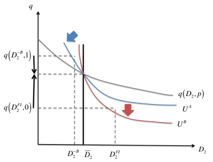
Figure 9: Pooling equilibrium with a common debt ceiling.
