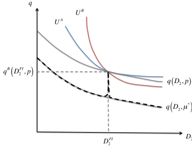
Figure 3: A pooling equilibrium at D_2^{FI} .
