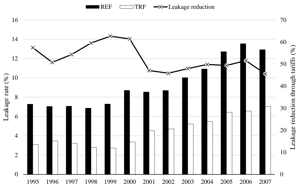
Figure 3: Leakage rates under REF and TRF (left axis) and percentage leakage reduction through tariffs (right axis)
