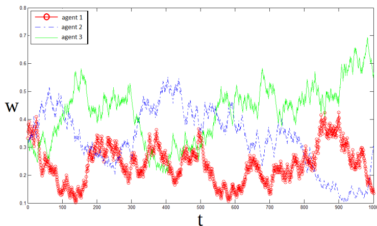
Figure 9: Simulation of the evolution of wealth shares for 1000 periods.
