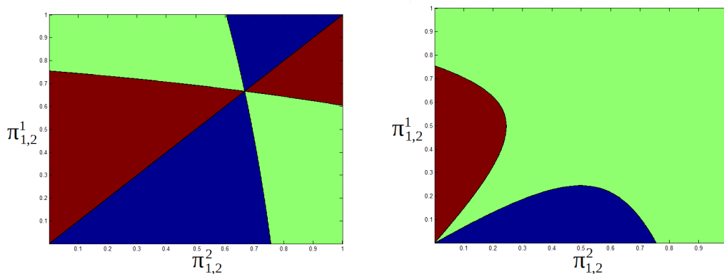
Figure 6: Areas of dominance and survival. Red: agent 1 dominates, blue: agent 2 dominates, green: long-run heterogeneity. Left plot: incomplete markets. Right plot: complete markets.
