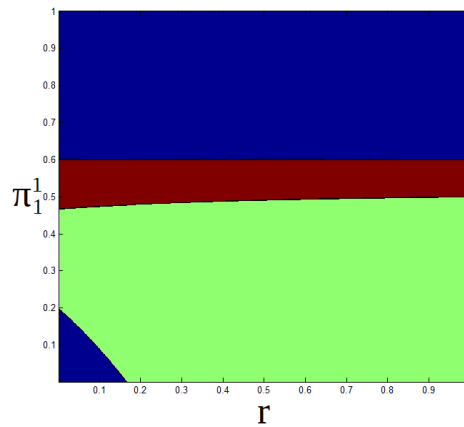
Figure 5: Areas of dominance and survival. Red: agent 1 dominates, blue: agent 2 dominates, green: long-run heterogeneity. \delta = 0.5
