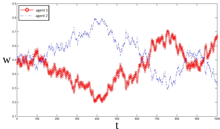
Figure 3: Simulation of the evolution of wealth shares for 1000 periods.
