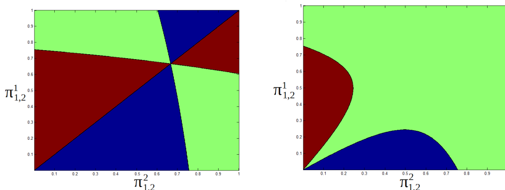
Figure 6: Areas of dominance and survival. Red: agent 1 dominates, blue: agent 2 dominates, green: long-run heterogeneity. Left plot: incomplete markets. Right plot: complete markets.
