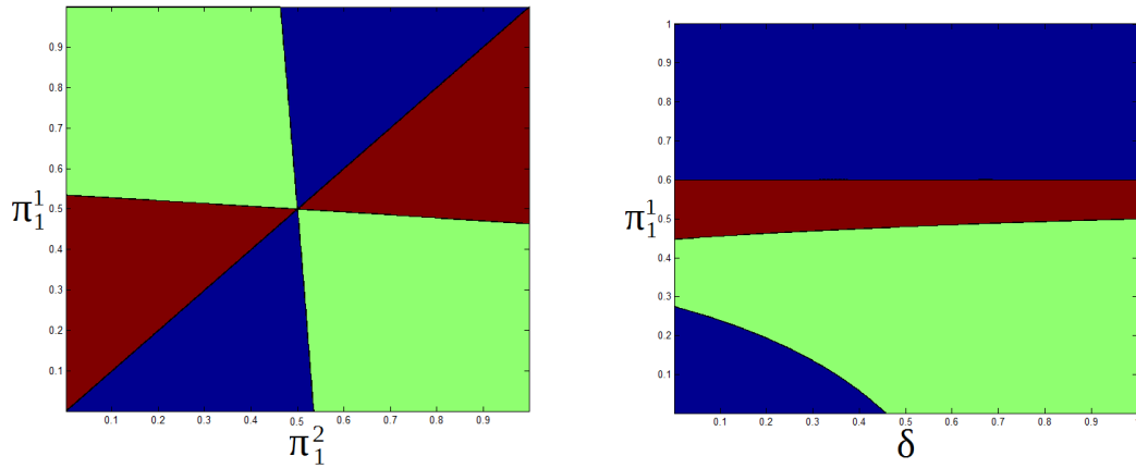
Figure 4: Areas of dominance and survival. Red: agent 1 dominates, blue: agent 2 dominates, green: long-run heterogeneity. r = 0.2
