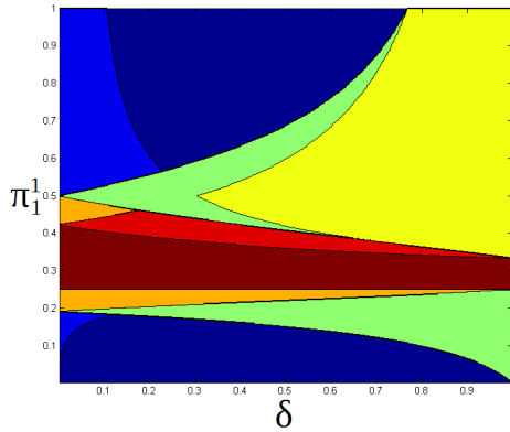
Figure 8: Areas of dominance and survival. Red: agent 1 survives; Dark Red: agent 1 dominates; Blue: agent 1 vanishes; Dark Blue: only agent 2 and agent 3 survive; Green: at least two agents survive; Yellow: all three agents survive; Orange: unknown.
