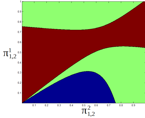
Figure 7: Areas of dominance and survival. Red: agent 1 dominates, blue: agent 2 dominates, green: long-run heterogeneity. Complete markets.
