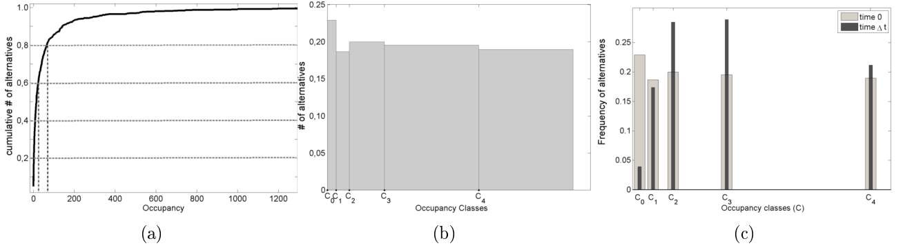
Figure 2: Binning procedure
