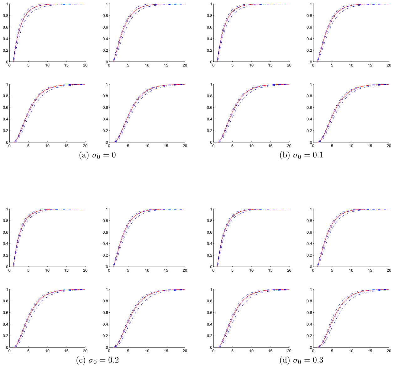
Figure VII: Distributions of Unobserved Auction Heterogeneity: Strong Selection. Red solid line: True distribution. Blue dot-dash lines: 2.5%, 50%, 97.5% quantiles of the estimator. In each sub-figure, the first row is for 2 and 3-bidder auctions, and the second row is for 4 and 5-bidder auctions.
