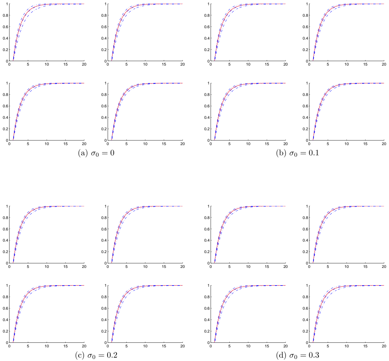
Figure III: Distributions of Unobserved Auction Heterogeneity. No Selection (DGP 1). Red solid line: True distribution. Blue dot-dash lines: 2.5%, 50%, 97.5% quantiles of the estimator. In each sub-figure, the first row is for 2 and 3-bidder auctions, and the second row is for 4 and 5-bidder auctions.
