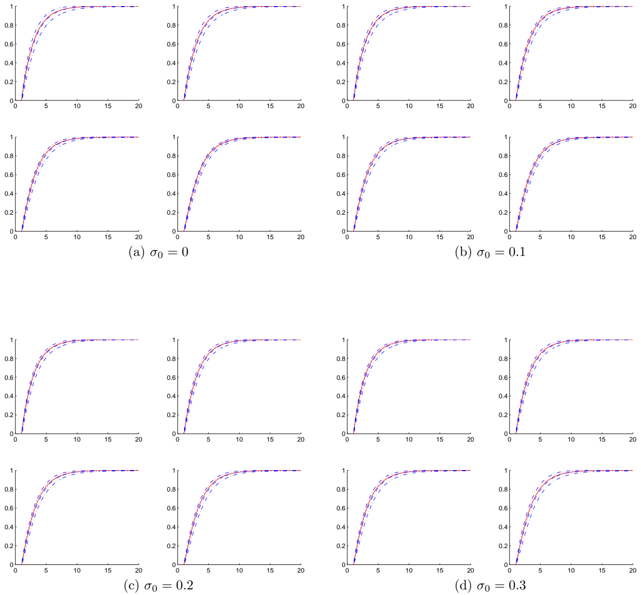
Figure V: Distributions of Unobserved Auction Heterogeneity: Weak Selection (DGP 2). Red solid line: True distribution. Blue dot-dash lines: 2.5%, 50%, 97.5% quantiles of the estimator. In each sub-figure, the first row is for 2 and 3-bidder auctions, and the second row is for 4 and 5-bidder auctions.
