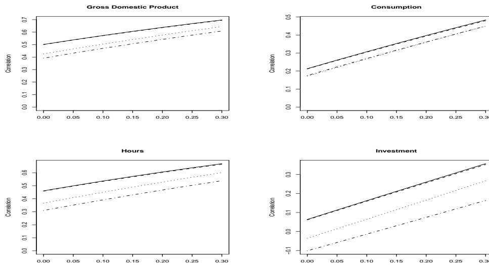
Figure 8 Cross-Country Correlation Sensitivity to Correlated Technologies
