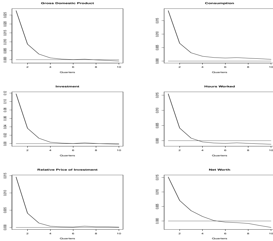
Figure 5 Impulse Responses to Home Country Risk Shock: Foreign Country
