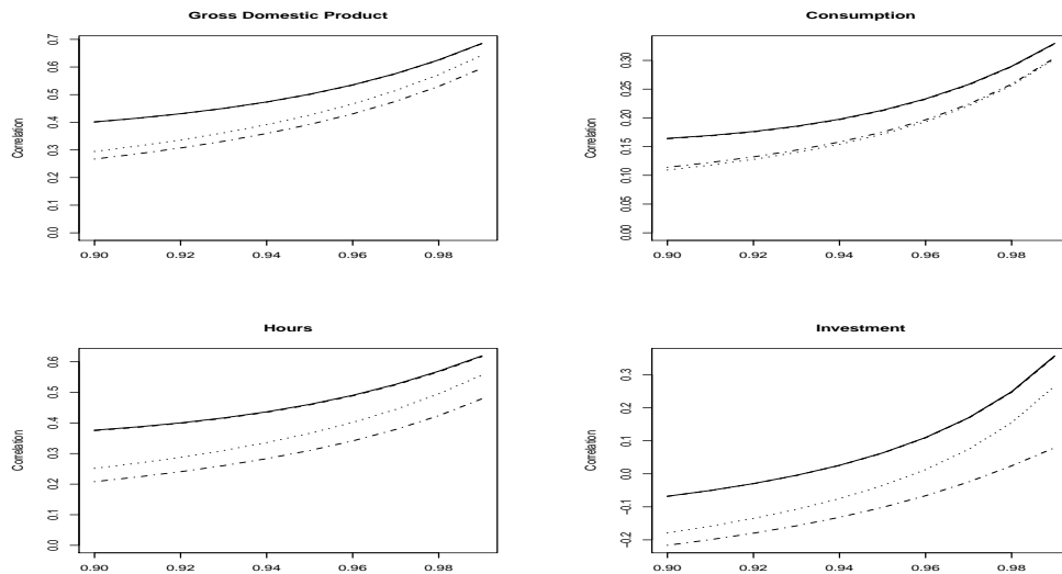
Figure 10 Cross-Country Correlation Sensitivity to Technology Persistence
