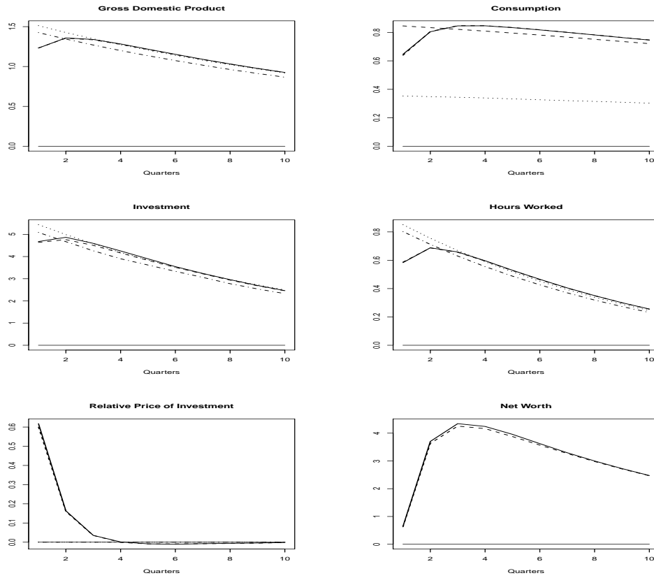
Figure 1 Impulse Responses to Home Country TFP Shock: Home Country
