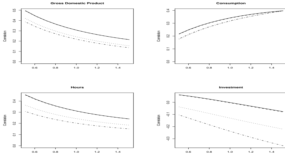
Figure 7 Cross-Country Correlation Sensitivity to the Elasticity of Substitution
