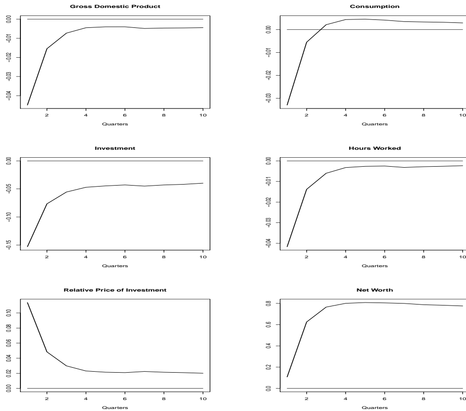
Figure 4 Impulse Responses to Home Country Risk Shock: Home Country
