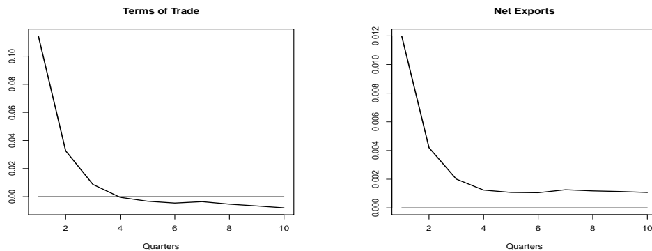
Figure 6 Impulse Responses to Home Country Risk Shock: Home Country's Terms of Trade and Net Exports
