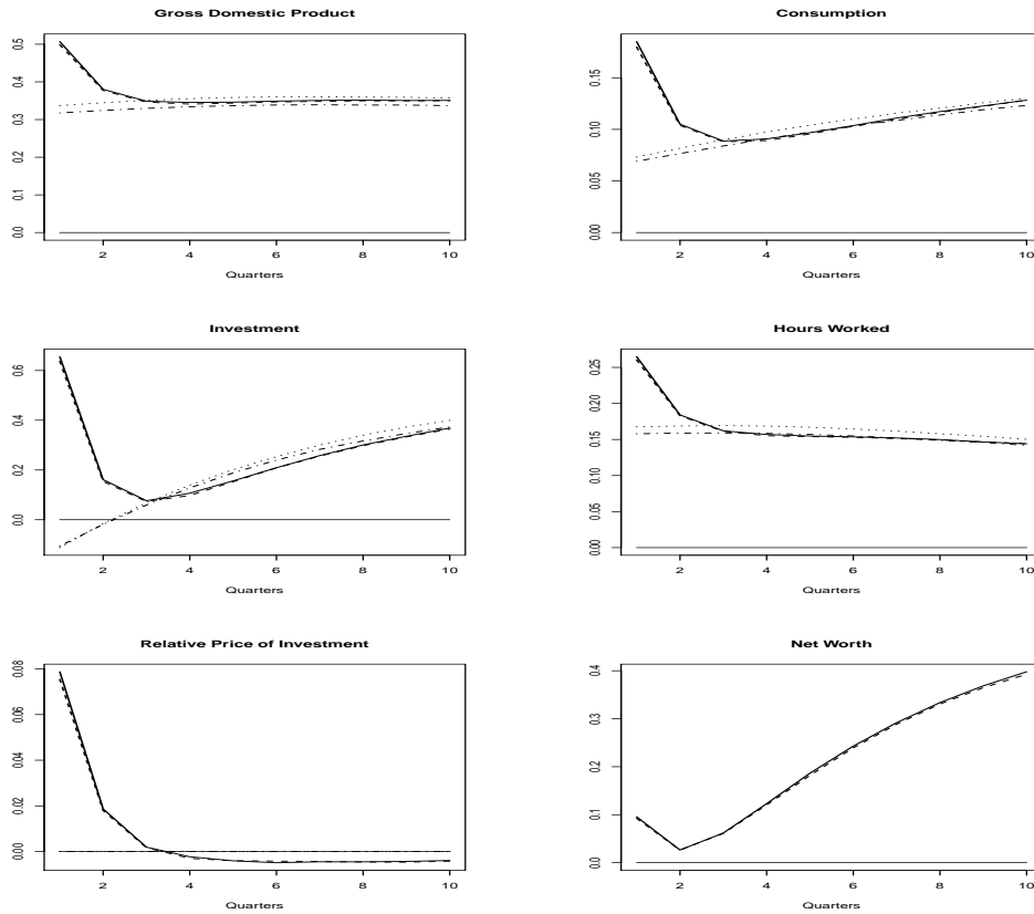
Figure 2 Impulse Responses to Home Country TFP Shock: Foreign Country
