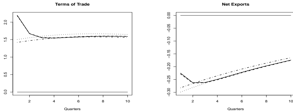
Figure 3 Impulse Responses to Home Country TFP Shock Home Country's Terms of Trade and Net Exports
