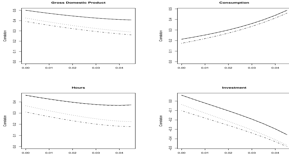
Figure 9 Cross-Country Correlation Sensitivity to Technology Spillovers
