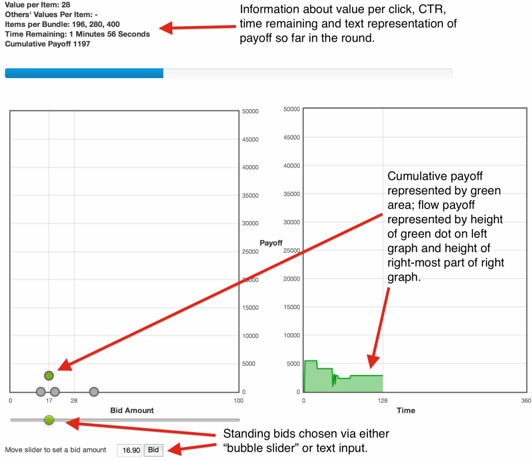
Figure 2: User Interface.
