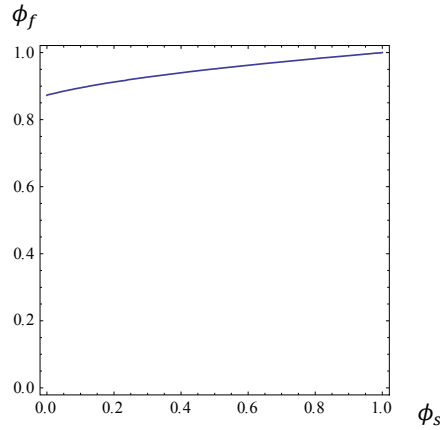
Fig. 1 Symmetry breaking
