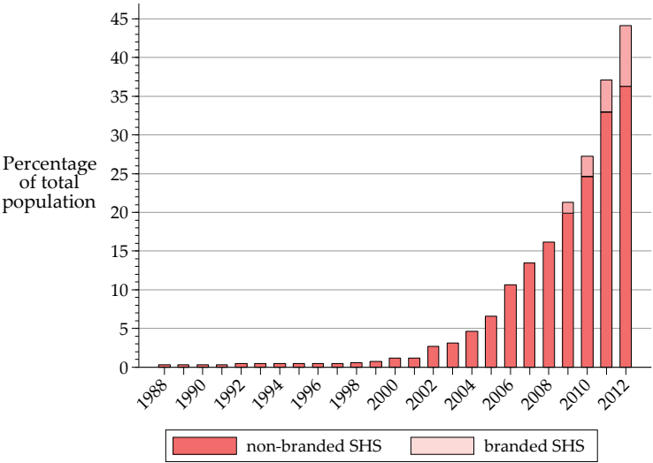
Figure 2: Cumulative SHS take-up over time
