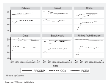
Figure 1. Real GDP, CO 2 emissions and energy use in the GCC (1960–2013, log-scale).
