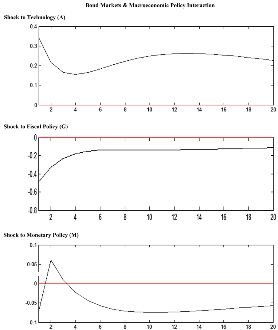
Figure 10. Impulse response function analysis.
