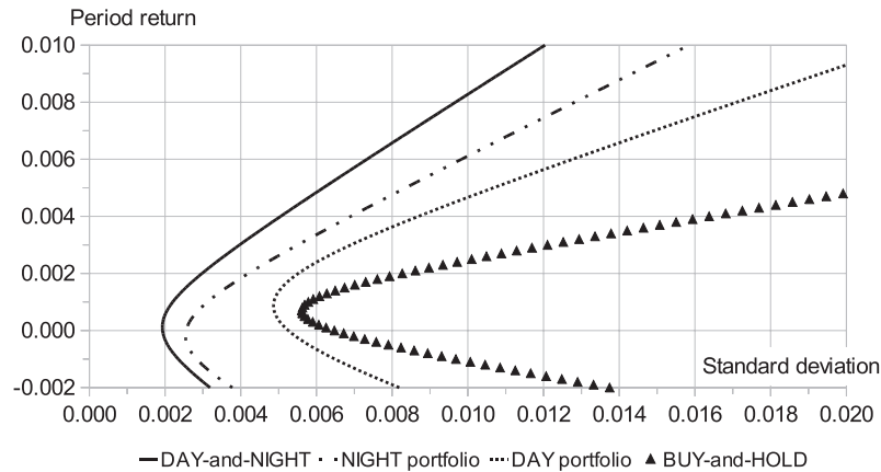
Figure 4. The plot of optimal portfolios (efficient frontiers) for the four strategies under consideration.
