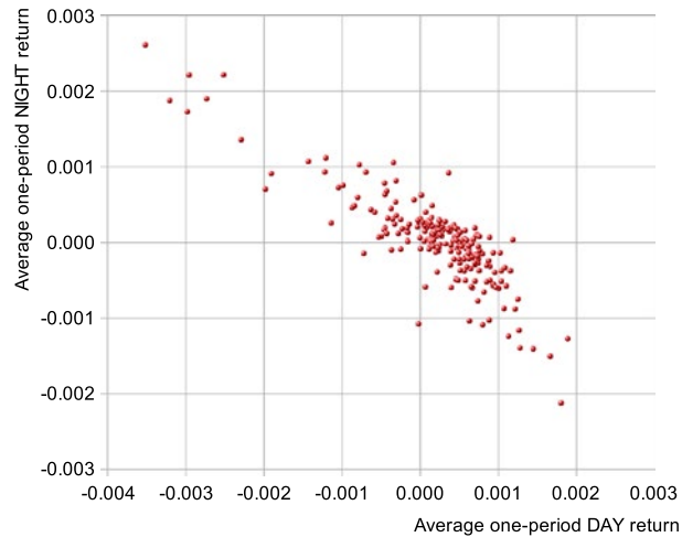
Figure 2. The scatter plot of the relationship between average one-period DAY (horizontal axis) and average one-period NIGHT returns (vertical axes) of a stock.
