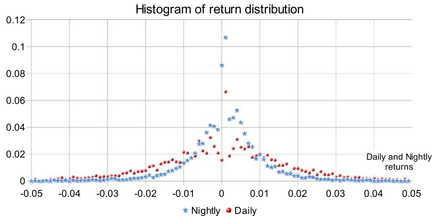
Figure 1. Comparison of DAY and NIGHT returns.
