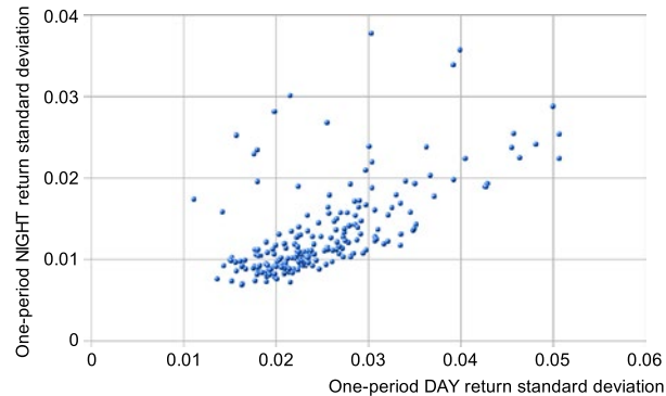
Figure 3. The scatter plot of the relationship between standard deviations of DAY (horizontal axis) and NIGHT returns (vertical axes).
