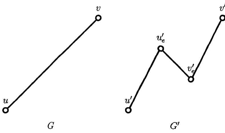
Figure 2: Reduction of the simple perfect b -matching problem to the perfect b -matching problem
