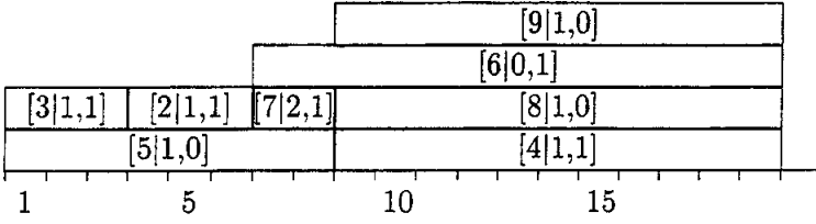
Figure 2: Gantt-Charts of Partial Schedules
