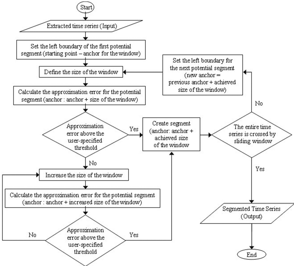
Figure 8. The flowchart for the Sliding Window algorithm
