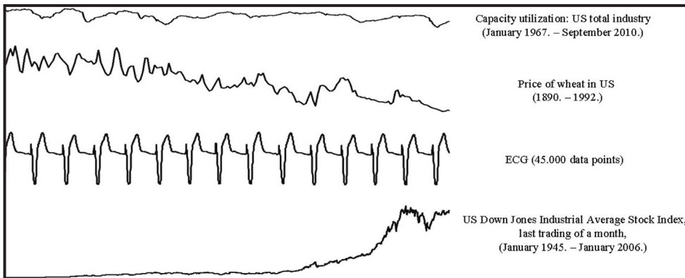
Figure 1. Examples of time series
