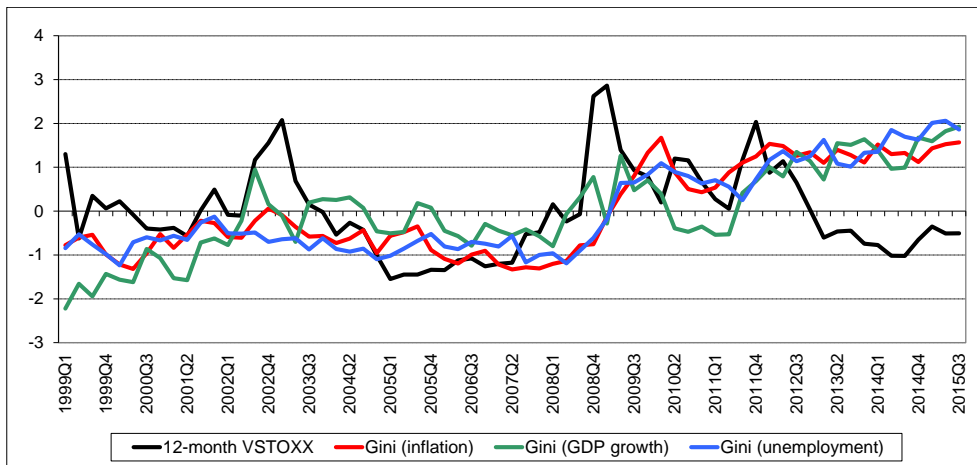
Figure 10: Comparison between the standardised VSTOXX indices and the standardised SPF-based uncertainty measures from density forecasts one and two years ahead
