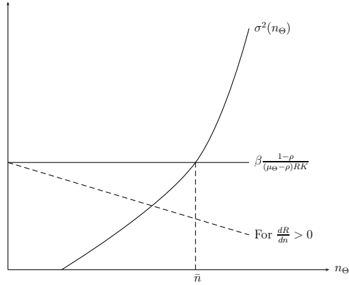
Figure 1: Granularity bound \bar{n}[\mu_{\Theta}, r, \underline{R}, \underline{K}] .
